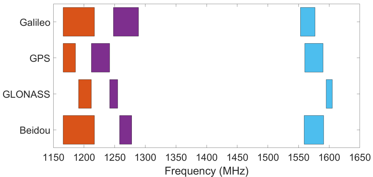
Figure 1: GNSS Frequencies
